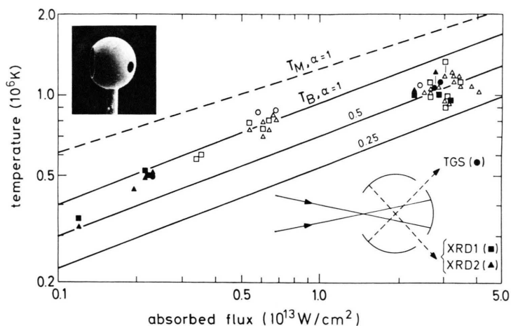
Fig. 1. Laser heating of gold cavities of 1 mm diameter ( S_L below 10^{13} \text{ W cm}^{-2} ) and 250–300 \mu\text{m} diameter ( S_L above 10^{13} \text{ W cm}^{-2} ). Full and open experimental points correspond to measurements at \lambda = 0.44 \mu\text{m} and \lambda = 1.3 \mu\text{m} , respectively.
